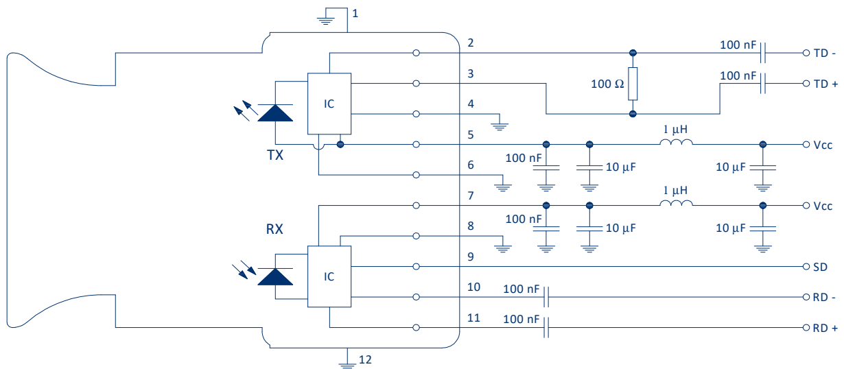
FIGURE 1 Recommended circuit layout for the OptoLock® transceiver
