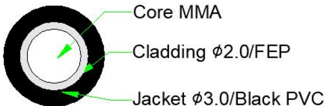
TX-SCC2000-1/3.0 Structure diagram
