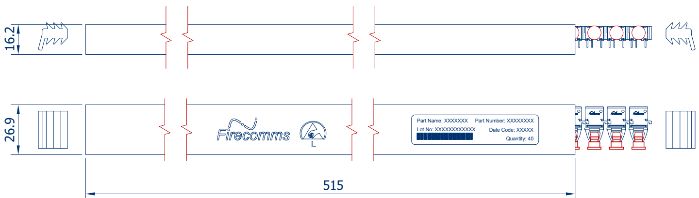
FIGURE 5 Packing tube for Firecomms RedLink® horizontal connectors
