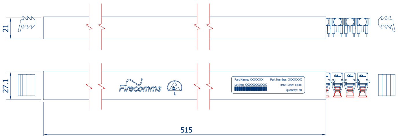
FIGURE 9 Packing tube for Firecomms RedLink® tilted connectors
