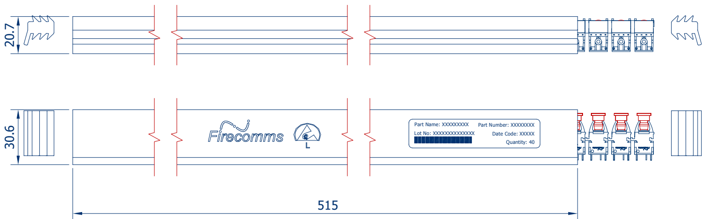
FIGURE 7 Packing tube for Firecomms RedLink® vertical connectors
