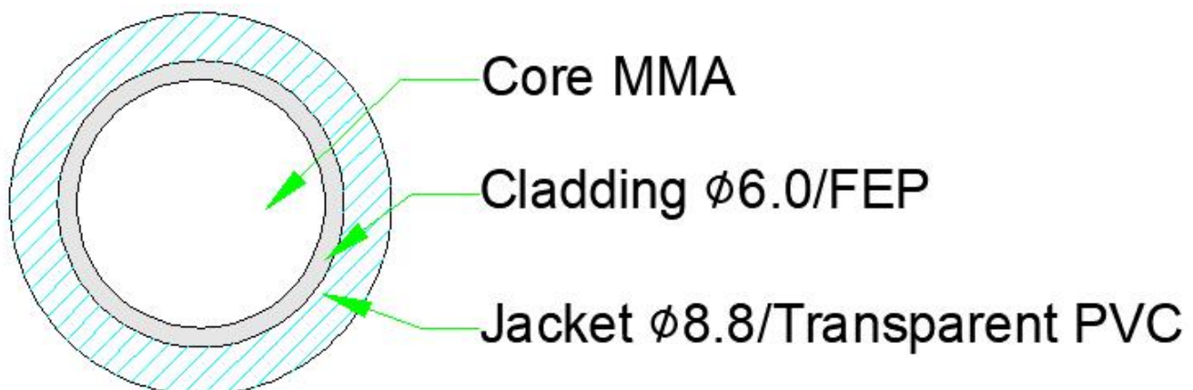
TX-SCC6000-1/8.8T Structure diagram
