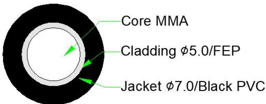
TX-SCC5000-1/7.0 Structure diagram
