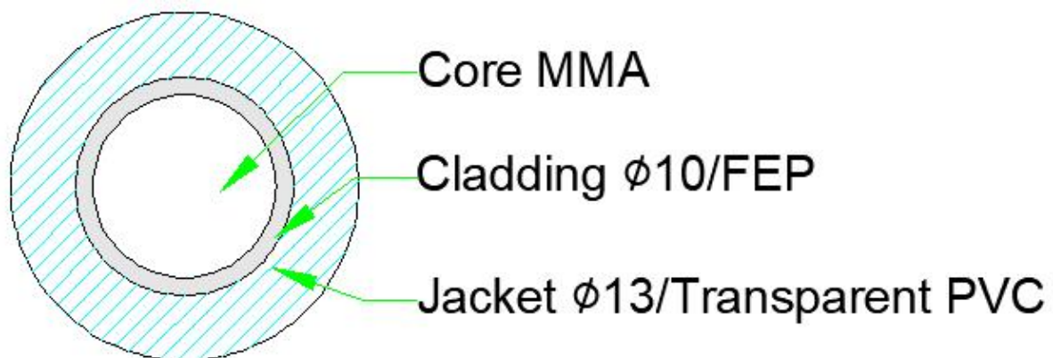
TX-SCC10000-1/13T Structure diagram
