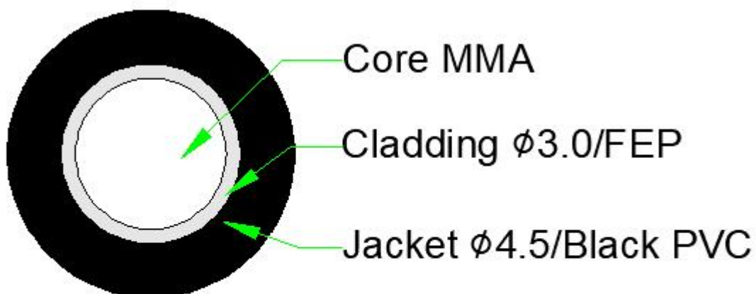
TX-SCC2500-1/4.0 Structure diagram
